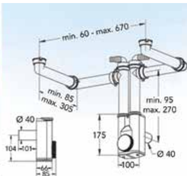
Siphon double Space Saver
